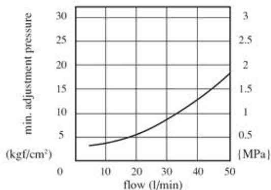
MB☆-01-☆-B-10T flow-min. pressure characteristic
