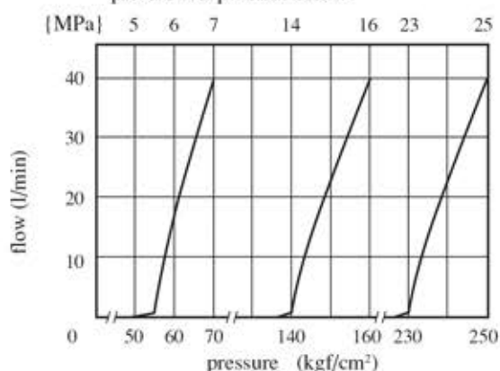
MB☆-01-☆-10T pressure drop characteristic
