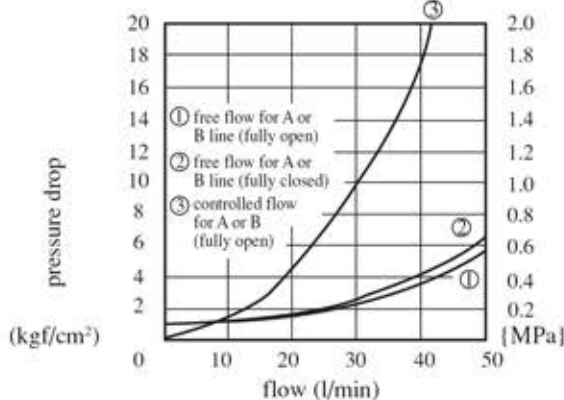
MSW-01-X-10T MSW-01-Y-10T pressure drop characteristic
