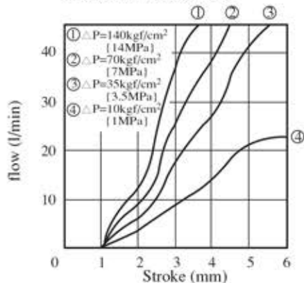
MS*-01-*-10T stroke-flow characteristic
